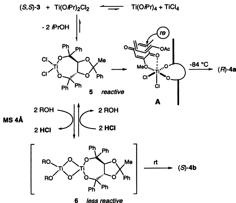
Scheme 1. A proposed reaction pathway
